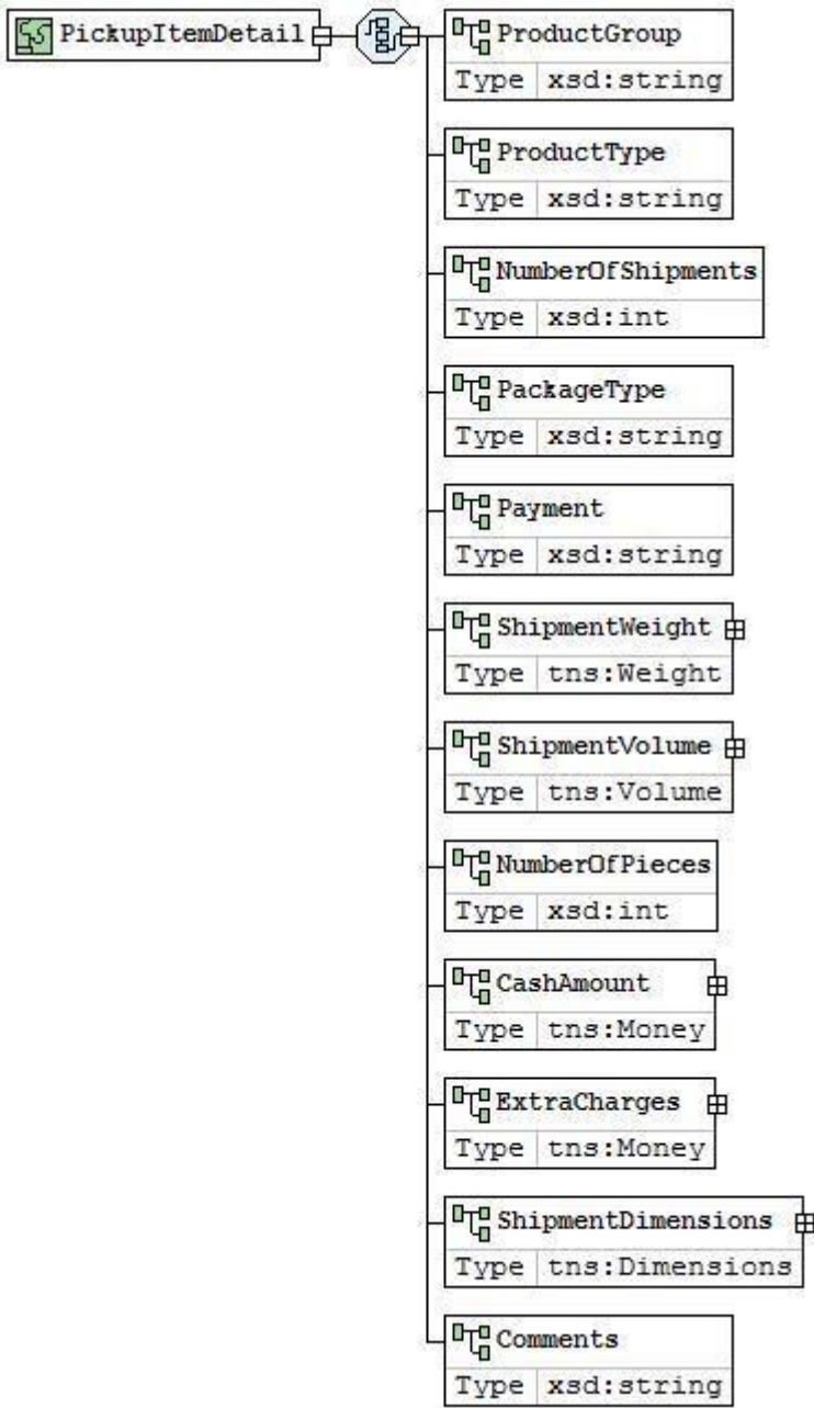
Fig.25. Pickup Item Details Structure Diagram
